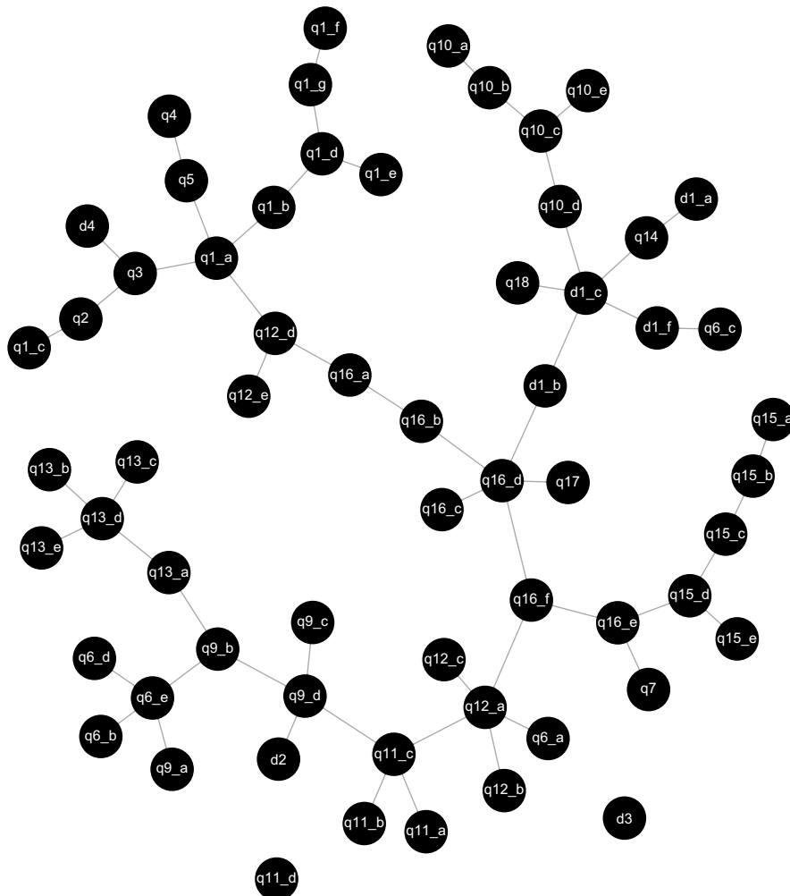
Figure 1: The minimum BIC forest
