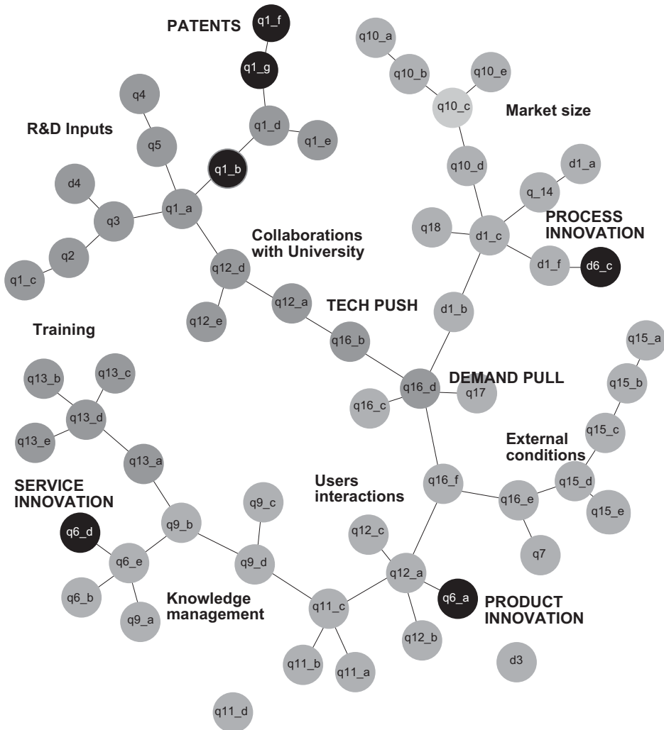
Figure 2: The minimum BIC forest with labels
